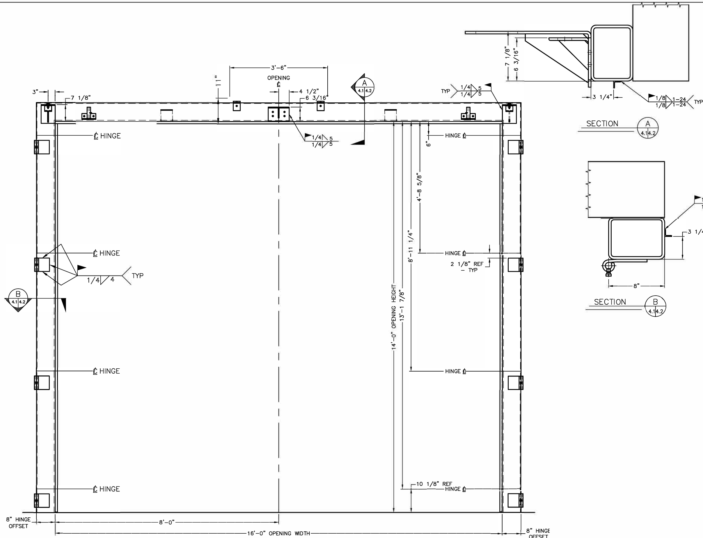
HARDWARE PLACEMENT AND WELDING HINGE SIDE ELEVATION 8" HINGE OFFSET, TUBE STEEL FRAME
