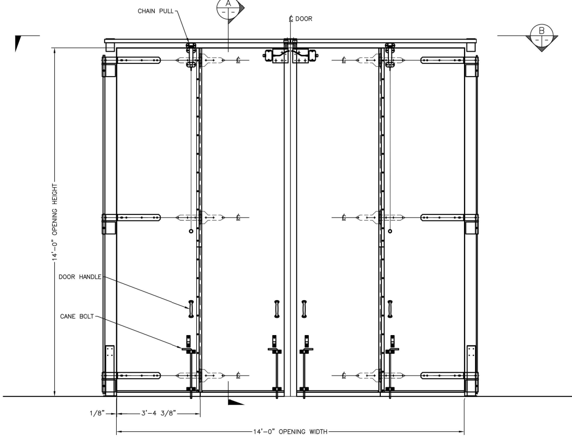
HYDRAULIC FOUR FOLD DOOR INTERIOR ELEVATION
