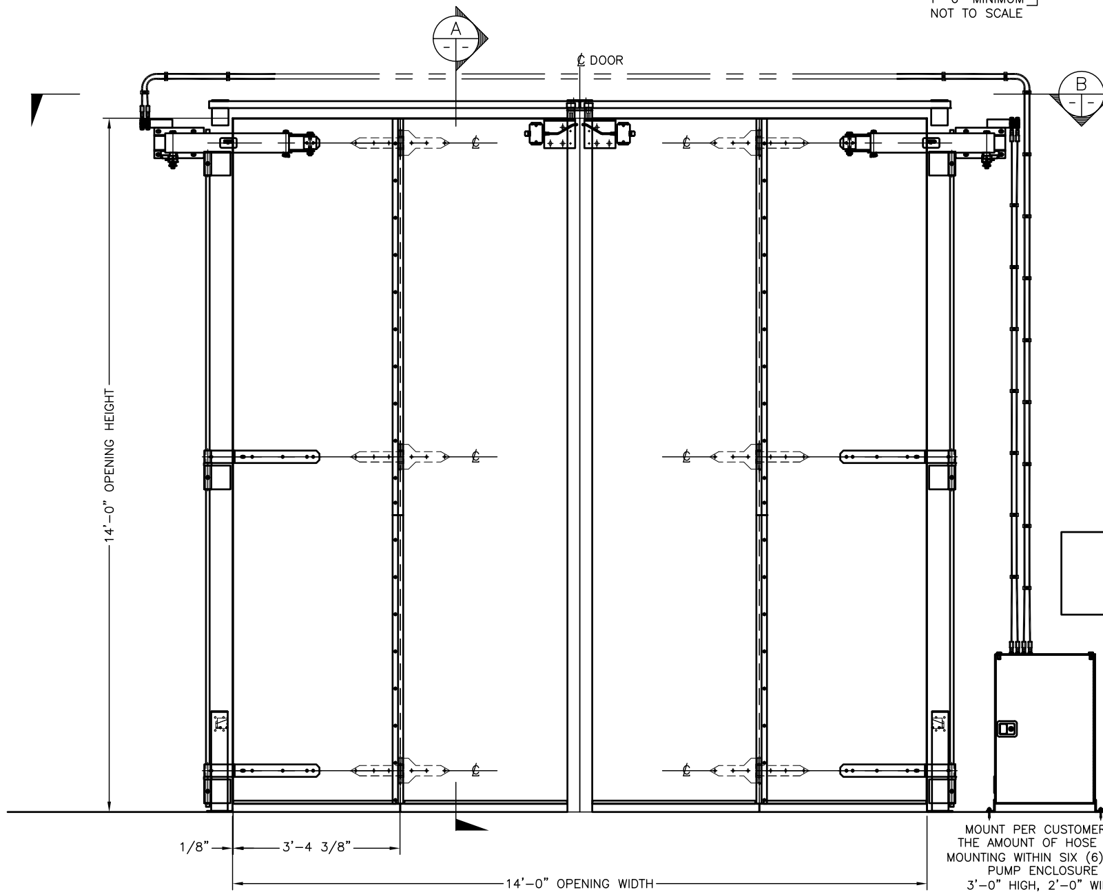
HYDRAULIC FOUR FOLD DOOR INTERIOR ELEVATION
