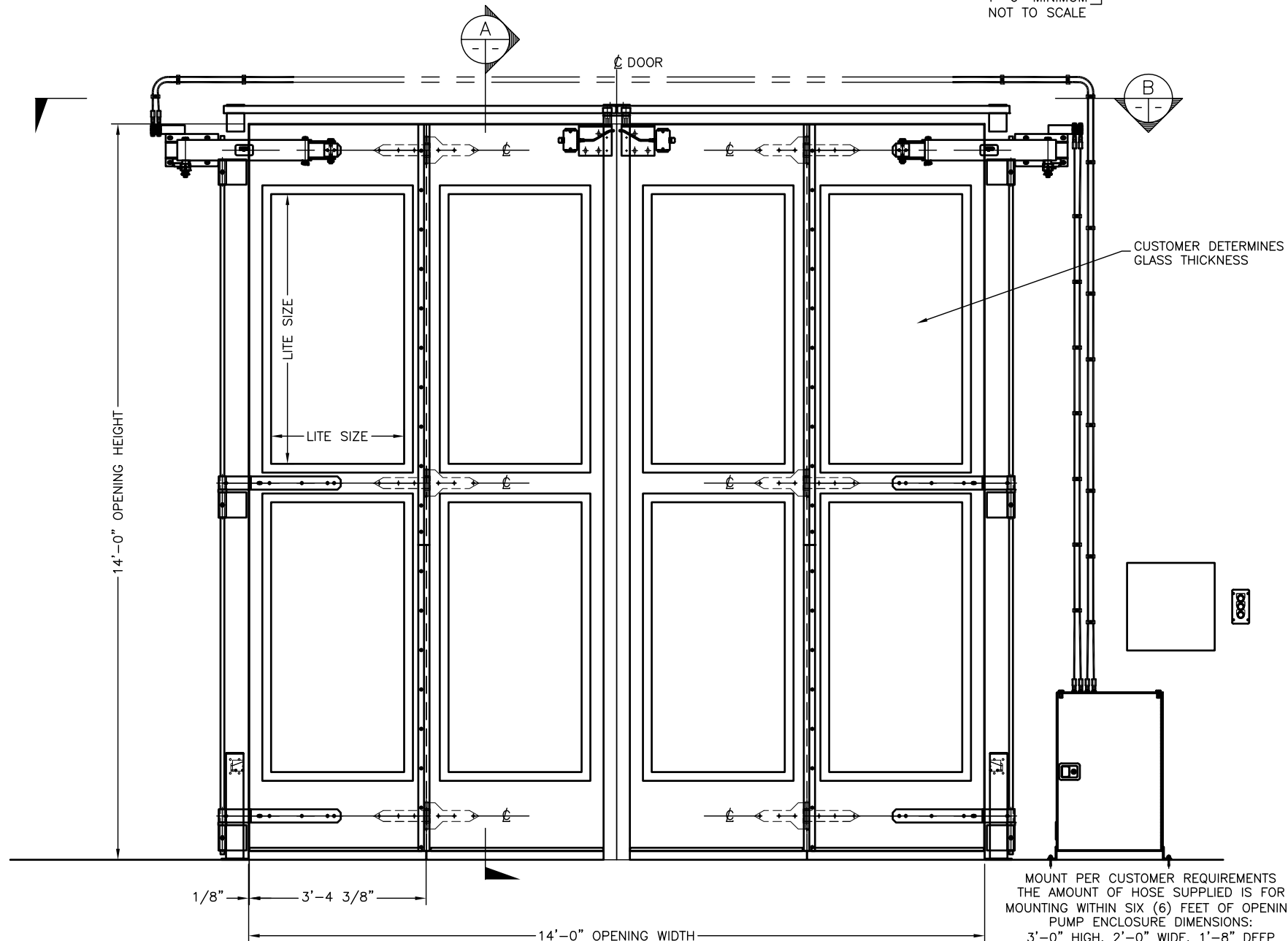
HYDRAULIC FOUR FOLD DOOR INTERIOR ELEVATION
