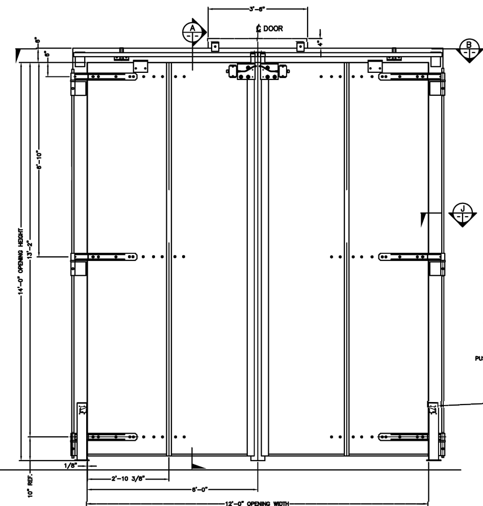
ELECTRIC FOUR FOLD DOOR INTERIOR ELEVATION - OPERATOR NOT SHOWN
