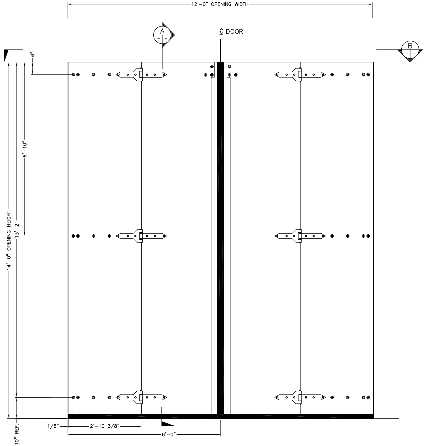
ELECTRIC FOUR FOLD DOOR EXTERIOR ELEVATION
