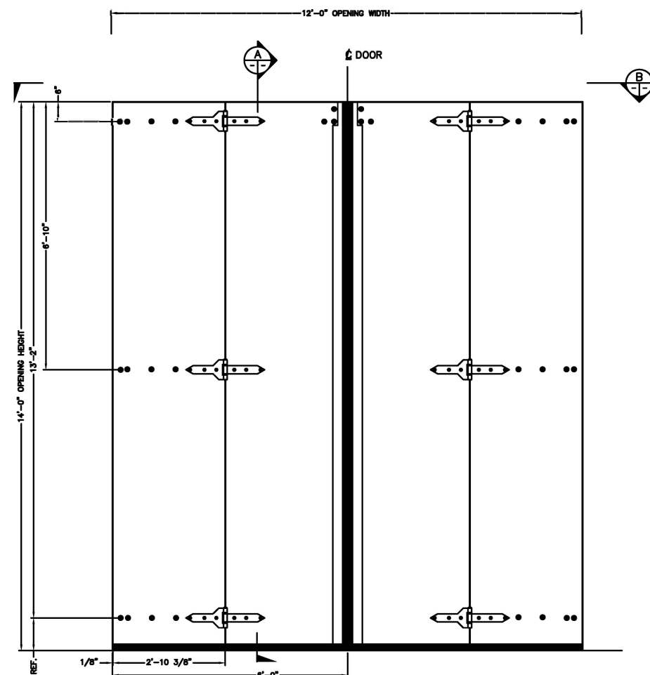
ELECTRIC FOUR FOLD DOOR EXTERIOR ELEVATION
