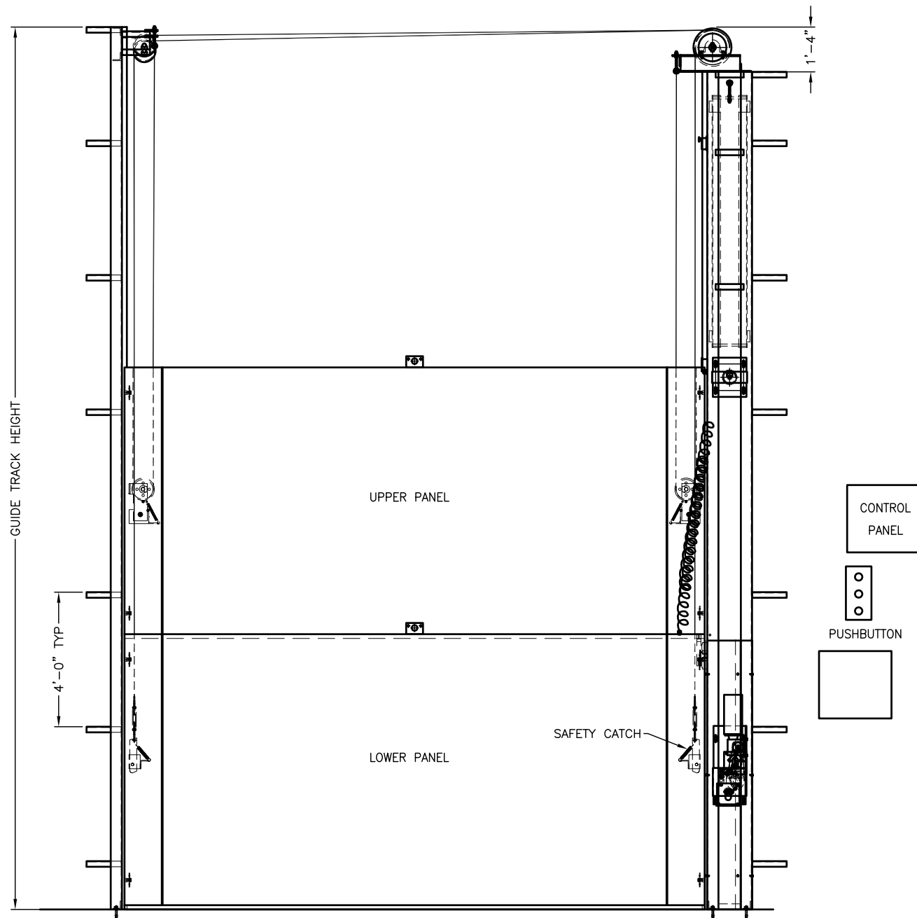
TWO LEAF VERTICAL LIFT DOOR INTERIOR ELEVATION
