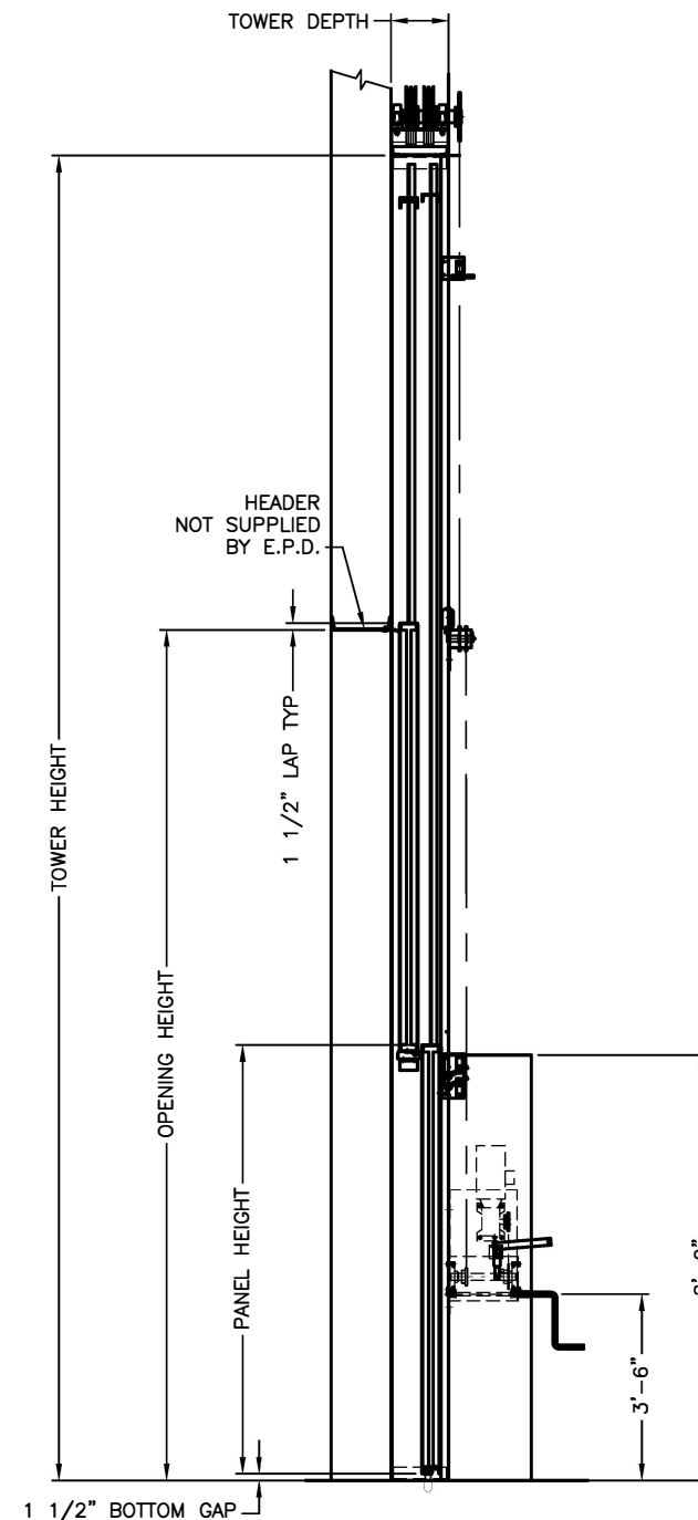
SECTION
