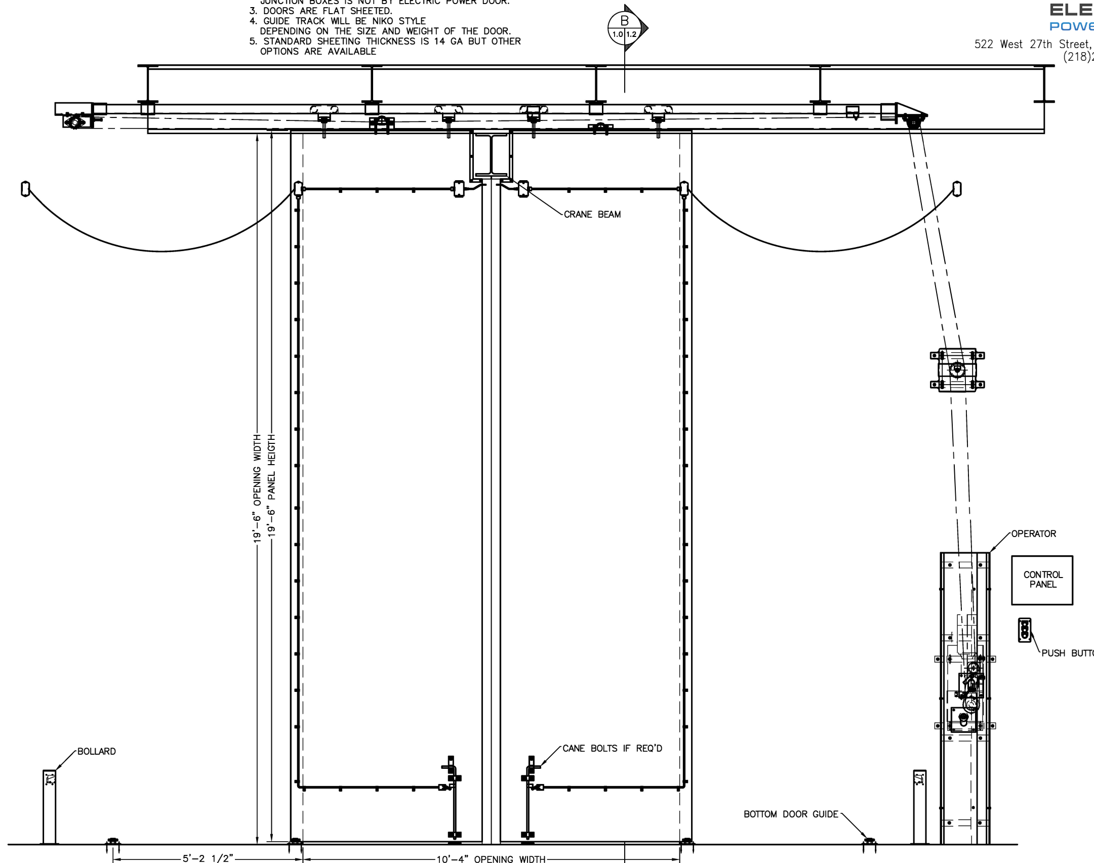
INTERIOR ELEVATION
