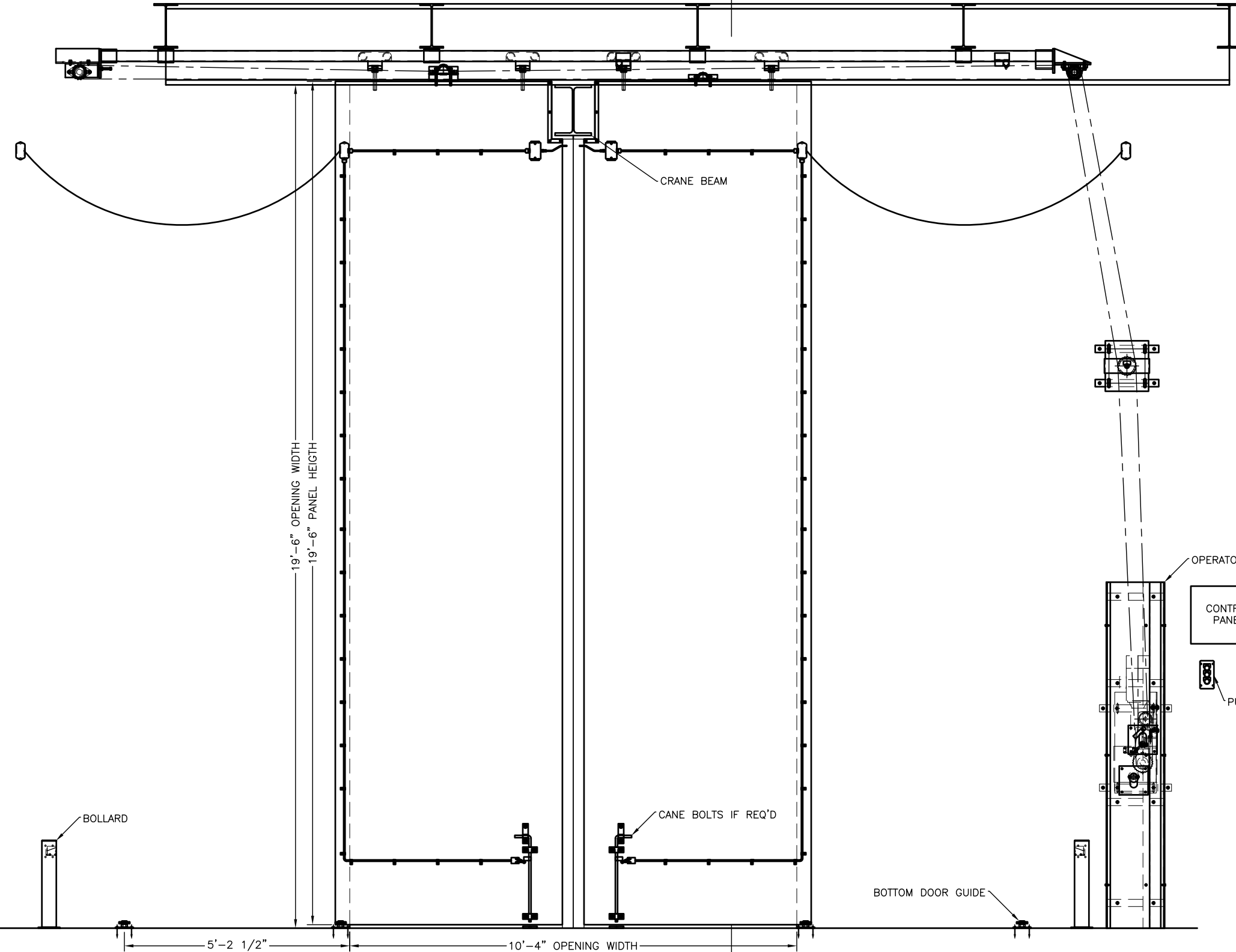
INTERIOR ELEVATION
