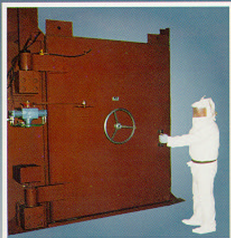
HIGH-RANGE BLAST RESISTANT DOOR
